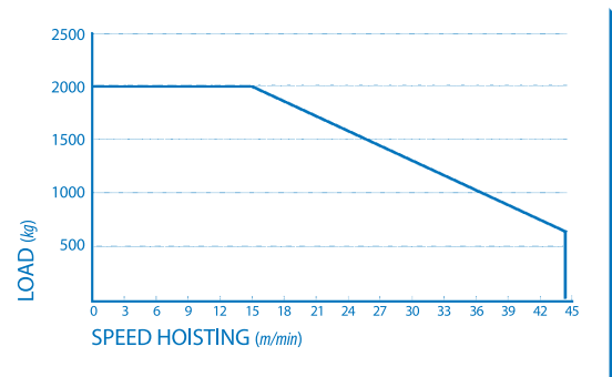
SPEED DIAGRAM
