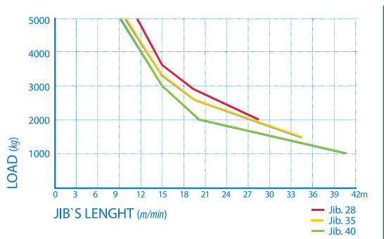
LOAD DIAGRAM
